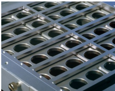
DESK_GmbH-B022-NIM-Cassetten-im-Überrahmen2
