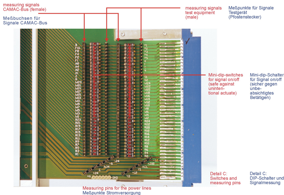
CAMAC-Expander-B3
